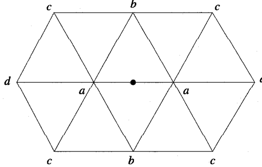
Figure 9: 1. Four-point stencil. 2. Eight-point stencil (Butterfly scheme.)
