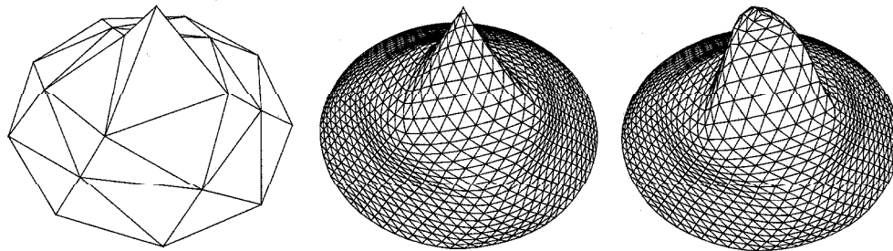
Figure 1: On the left an input control mesh with a vertex of valence 3. In the middle the result after several levels of subdivision using the Butterfly scheme. The surface loses smoothness around the vertex of valence 3. On the right the result achieved in the same situation with our modified scheme. The behavior around the extraordinary vertex remains smooth and no cusp is formed.
