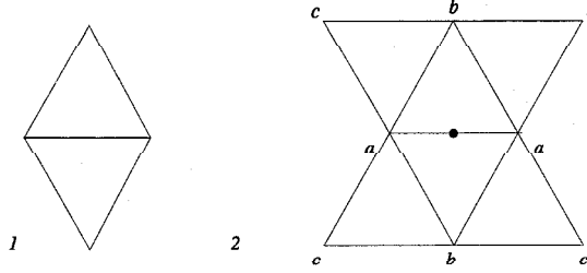
Figure 9: 1. Four-point stencil. 2. Eight-point stencil (Butterfly scheme.)
