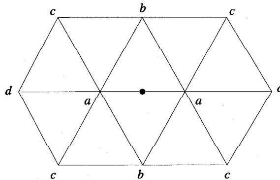
Figure 3: Ten-point stencil.
