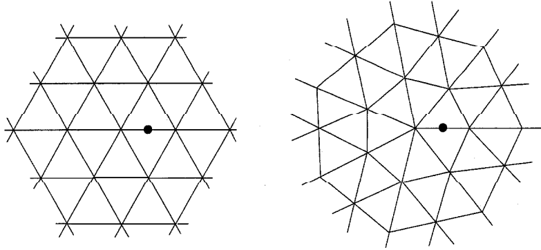
Figure 2: On the left a regular neighborhood in which all vertices have valence 6. On the right an example of a K = 7 vertex. In both cases the dot represents a typical midpoint for which we seek to compute a new value. In the regular case the Butterfly stencil is used, while in the K \neq 6 a separate analysis is performed leading to a local modification of the weights.
