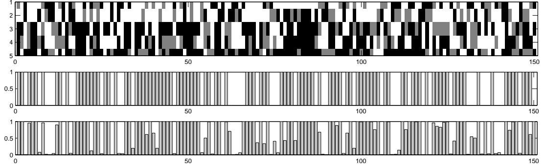
Figure 20.4: Top: Data from questionnaire responses. 150 people were each asked 5 questions, with ‘yes’ (white) and ‘no’ (black) answers. Gray denotes that the absence of a response (missing data). This training data was generated by a two component product of Bernoulli model. Missing data was simulated by randomly removing values from the dataset. Middle: the ‘correct’ h values sampled from the data. A ‘0’ denotes h^n = 1 and ‘1’ denotes h^n = 2 . Bottom: The estimated p(h_i^n = 2 | \mathbf{v}^n) values.
