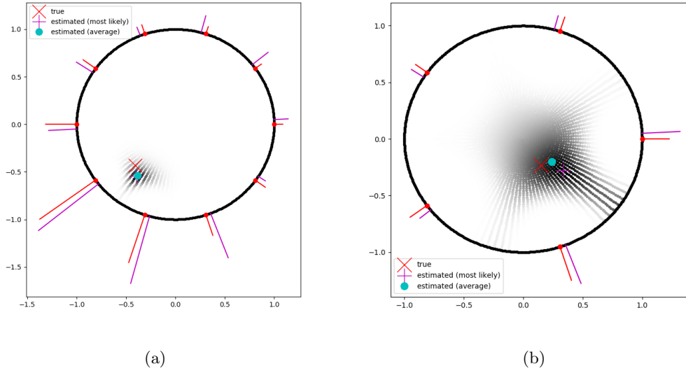
Figure 1.2: The posterior distribution for the location of the explosion (darker corresponds to a higher probability). This is based on a spiral coordinate system (see earthquake.jl ) with \sigma = 0.2 . The red points are the locations of the surface sensors. The observed (noisy) measurements at each sensor are represented by the magenta lines, and the true (unknown) blast values are denoted by the red lines. (a) Using 10 sensors. (b) Using 5 sensors. Note how the uncertainty in the posterior is larger in the case of having fewer sensors.
