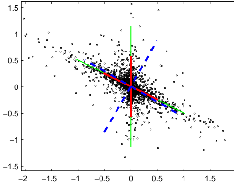
Figure 21.10: Latent data is sampled from the prior p(x_i) \propto \exp(-5\sqrt{|x_i|}) with the mixing matrix \mathbf{A} shown in green to create the observed two dimensional vectors \mathbf{y} = \mathbf{A}\mathbf{x} . The red lines are the mixing matrix estimated by ica.m based on the observations. For comparison, PCA produces the blue (dashed) components. Note that the components have been scaled to improve visualisation. As expected, PCA finds the orthogonal directions of maximal variation. ICA however, correctly estimates the directions in which the components were independently generated. See demoICA.m .
