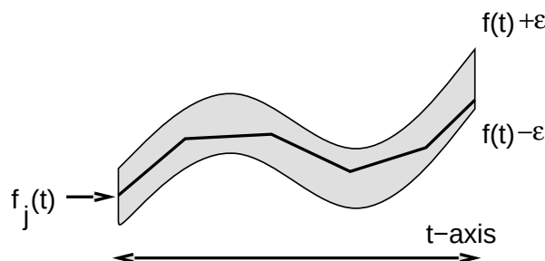
Figure 3.2 Uniform convergence
