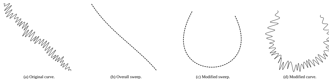
Figure 9.2 Multi-resolution editing
