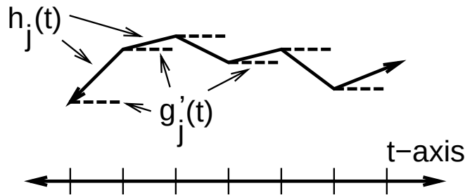
Figure 5.1 Convergence of g'_j(t) and h_j(t)
