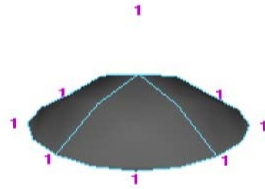
Level 1 vertices.
