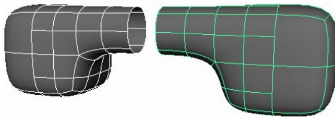
After Attach
