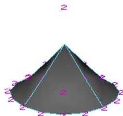
Level 2 vertices.
