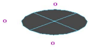
Level 0 vertices.
