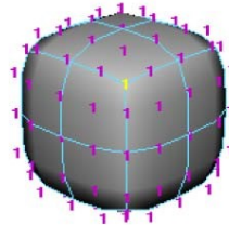
Level 1 vertices.
