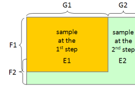
Figure 3: two-step labeling
