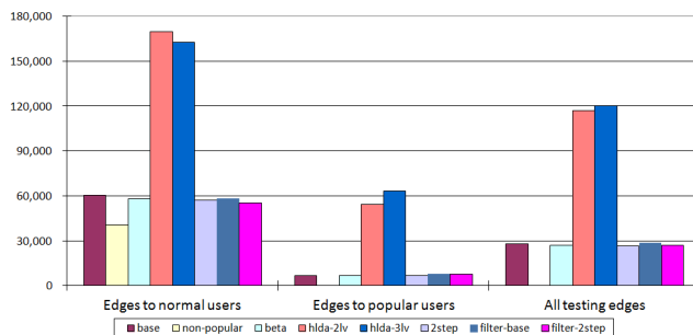
Figure 6: Perplexity comparison
