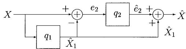
Fig. 9. Two-stage VQ.
